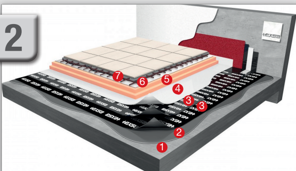
Inverted roof with heavy top protection TI-01-01.A2
