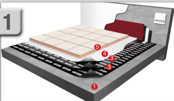
Inverted Roof with heave top protection TEXLOSA. NT-01-02.A2
