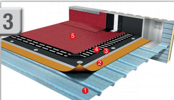
Metal deck Roof , Mechanical fixing or Adhered System NT-02-16.A2
